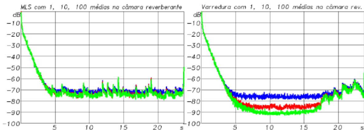
Fig. 10. Measurement of RIR with 12'' coaxial PA-speaker in a reverberant chamber. 1, 10 and 100 synchronous averages were performed. Left: with MLS, right: with sweep of identical coloration and energy. The curves are compressed to 1303 values, each of them representing the maximum of 805 consecutive samples.
